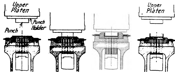
The successive positions assumed by the die and the punch in a complete cycle of the press
